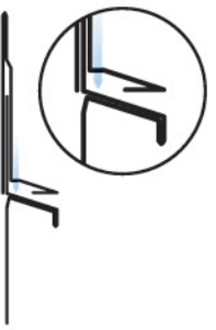
TWMSX: Tru-Weep™ M-Slide Expansion Joint®
