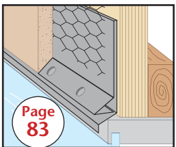
SSF: Stucco Screenshot Flashing (#3)
