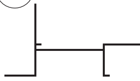
DS300: Drip Screed 3" Reveal
